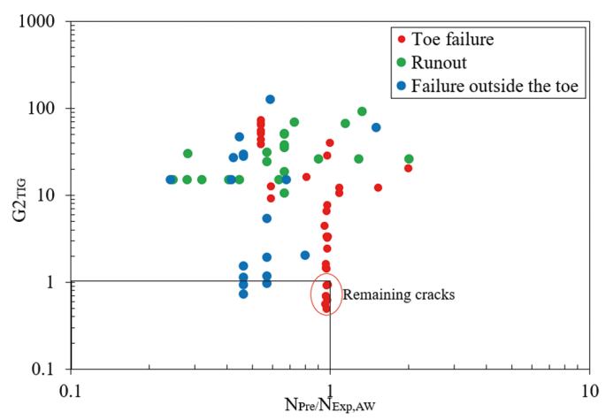
Fig. 20 Factor G2 plotted against the pre-fatigue cycles before TIG remelting normalized to the experimental mean as-welded life for groups 3.1, 3.2, 3.3 and 4.1
