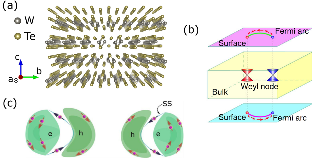
Figure 5.1: (a) Crystal lattice of T_d phase of WTe_2 . (b) Schematics of the Brillouin zone for Weyl semimetal. Adapted from ref. [261]. (c) Schematics of the Fermi surface of WTe_2 with electron, hole pockets and surface states (SS). Arrows indicate a peculiar spin texture. Adapted from ref. [264].
