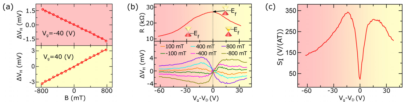
FIG. 4. Gate tunability of CVD graphene/h-BN Hall sensors at room temperature. (a) Output Hall voltage as a function of perpendicular magnetic field at gate voltages of \pm 40 V. (b) Back gate dependence of graphene resistance (top) and Hall voltage response at different perpendicular magnetic fields (bottom). V_D is the gate voltage corresponding to the Dirac point. (c) Absolute value of current-related sensitivity calculated from Hall voltage response as a function of gate voltage according to Eq. (2). The measurements at 75 K will be published elsewhere.
