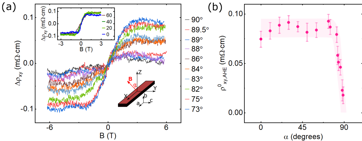
Figure 5.10: (a) Angle dependence of the Hall magneto resistivity \rho_{xy} in \text{ZrTe}_5 with angle range 73\text{-}90^\circ (main panel) and 0\text{-}60^\circ (top inset) at 4 K. The angle \alpha is swept in the a-b plane as shown in the bottom inset. The linear background contribution from the ordinary Hall effect is subtracted. (b) Angle dependence of the anomalous Hall contribution \rho_{xy,AHE}^0 . The colored background region is a guide to the eye.
