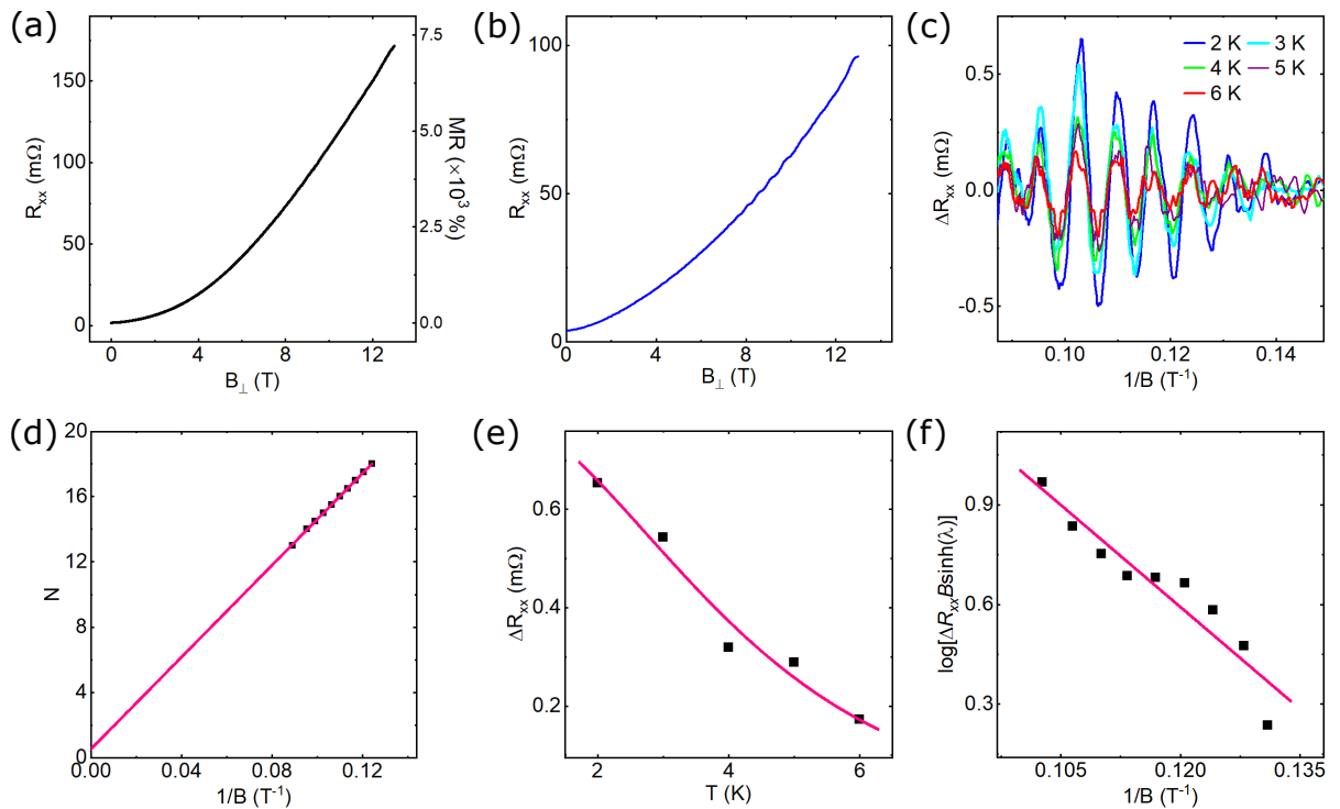
Figure 5.2: Electrical transport measurements in bulk \text{WTe}_2 sample. (a) Four-terminal resistance of the bulk channel R_{xx} and magneto resistance MR = R_{xx}(B_{\perp}) - R_{xx}(0)/R_{xx}(0) as a function of magnetic field B_{\perp} applied along the c -axis of the lattice at 2 K. (b) Magneto resistance with SdH oscillations at 2 K for another bulk channel. (c) Temperature dependence of the SdH oscillations in \text{WTe}_2 obtained from (a) after subtraction of the background signal. (d) Landau fan diagram of the Landau index N versus 1/B in the a - c plane. (e) Amplitude of the SdH oscillations \Delta R_{xx} as a function of temperature. The solid line is a fitting according to the equation 5.1. (f) Dingle plot at 2 K with fitting (solid line) according to the equation 5.2.
