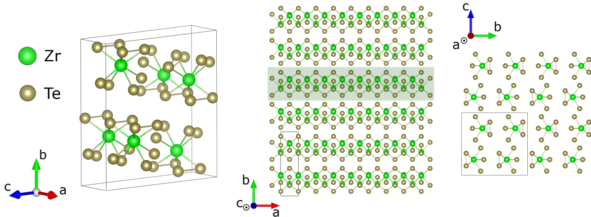
Figure 5.6: The crystal structure of \text{ZrTe}_5 . The solid line rectangulars and shaded region indicate single unit cells and quasi-1D chains, respectively.
