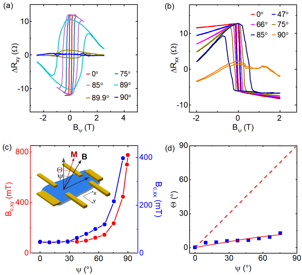
Figure 4.12: Angle dependence of the AHE in Fe 3 GeTe 2 . (a),(b) AHE measured for transverse ( R_{xy} ) and longitudinal ( R_{xx} ) magneto resistance at different angles. The data is shifted vertically. (c) Coercivity as a function of angle \psi obtained from (a) ( B_{c,xy} , red) and (b) ( B_{c,xx} , blue), respectively. Inset: schematics of the device configuration with noted angles between the out-of-plane direction and magnetization M (angle \Theta ) and magnetic field B (angle \psi ). (d) \Theta as a function of \psi (blue squares). The red dashed line represents the isotropic case \Theta = \psi while solid red line is a fitting according to Stoner-Wohlfarth model.
