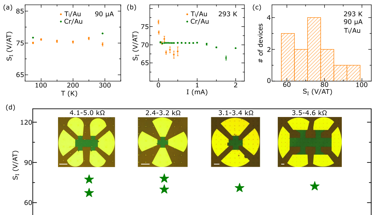
Figure 5. Current-related sensitivities ( S_T ) of graphene Hall elements. (a) Temperature dependence of S_T for Cr/Au and Ti/Au contacts measured at 90 \mu\text{A} current bias. (b) Current bias dependence of S_T for Cr/Au and Ti/Au contacts at room temperature. (c) Distribution of sensitivities S_T measured in 13 Hall elements with Ti/Au contacts at 90 \mu\text{A} current bias and at room temperature. The devices were selected from different parts of the wafer. (d) Sensitivities S_T for Hall sensors measured on devices with different size and geometry (Cr/Au contacts). Typical two-terminal resistances are shown with average resistivity value of \sim 75\text{--}100 \text{ k}\Omega\cdot\mu\text{m} (graphene sheet concentration \sim 8.5 \cdot 10^{12} \text{ cm}^{-2} ). Scale bars in the inset images are 60 \mu\text{m} .
