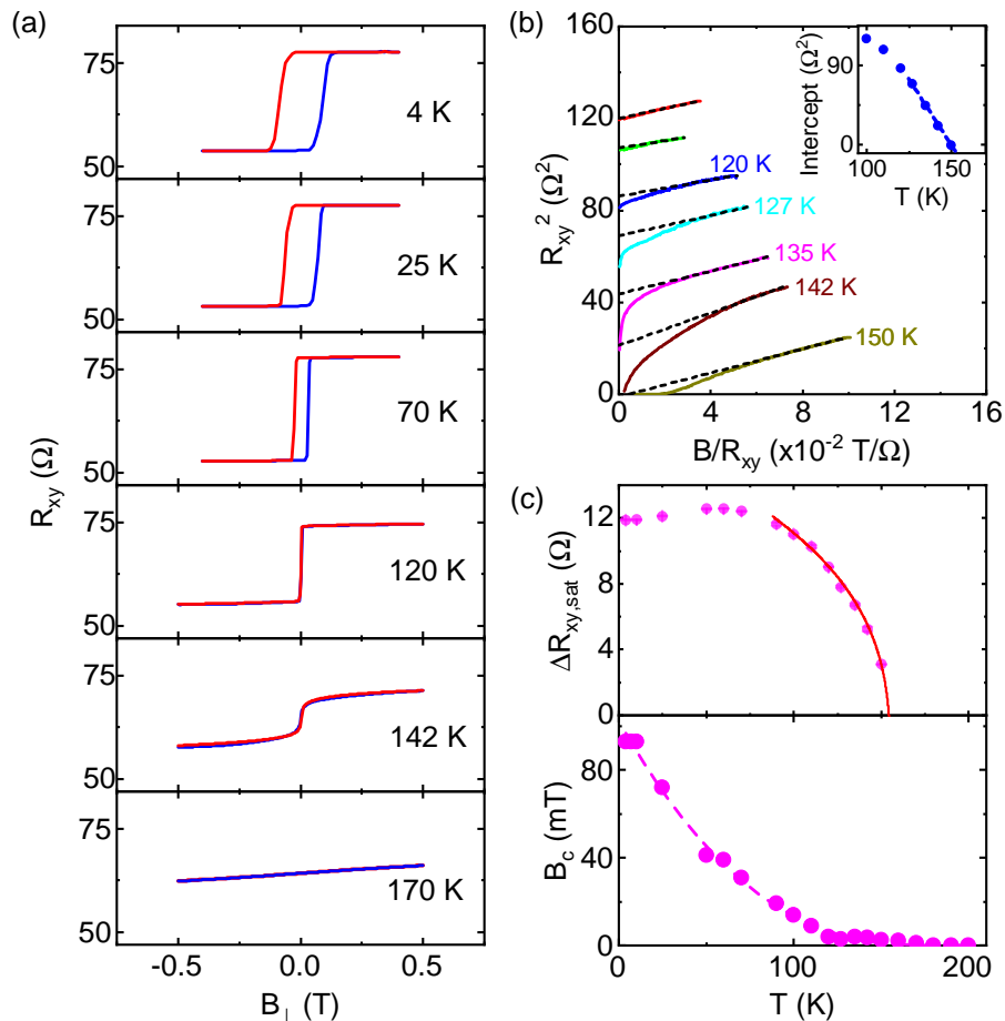
Figure 4.11: Temperature dependence of the AHE in \text{Fe}_3\text{GeTe}_2 . (a) AHE data measured in the \text{Fe}_3\text{GeTe}_2 Hall-bar device at different temperatures, as indicated. (b) Arrort plots of the AHE data. The inset shows the temperature dependence of the intercept. (c) Top panel: transverse resistance at saturation \Delta R_{xy,sat} , obtained after subtraction of the linear component. The red solid line is a fitting according to \Delta R_{xy,sat} \sim (1 - T/T_c)^\beta . Bottom panel: coercivity B_c as a function of temperature. The dashed line is a guide to the eye.
