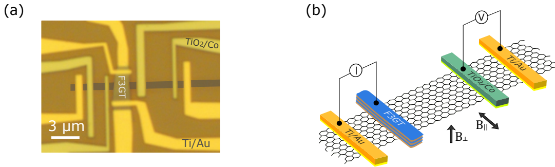
Figure 4.15: (a) Optical microscope picture of the \text{Fe}_3\text{GeTe}_2 /graphene heterostructure device. The graphene stripe is false-colored for clarity. (b) Schematics of the nonlocal measurement configuration for spin injection from the F3GT flake into the graphene channel and subsequent detection of spin current by conventional Co contacts.
