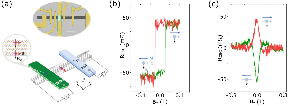
Figure 5.4: (a) Schematic of measurement geometry and false-colored device picture (the scale bar is 5 \mu\text{m} ) for electrical detection of charge-spin conversion in \text{WTe}_2 . The inset in the schematic show the spin polarization due to perpendicular current component K_z . (b) The nonlocal spin-valve measurement ( R_{CSC} = V_{CSC}/I , I is the bias current across the \text{WTe}_2 /graphene junction). (c) The corresponding Hanle spin precession signal observed for parallel and anti-parallel orientation of the injected spin ( s ) from \text{WTe}_2 and magnetization of ferromagnet ( M ) with positive and negative magnetic field B sweep directions at 300 K [Paper V].
