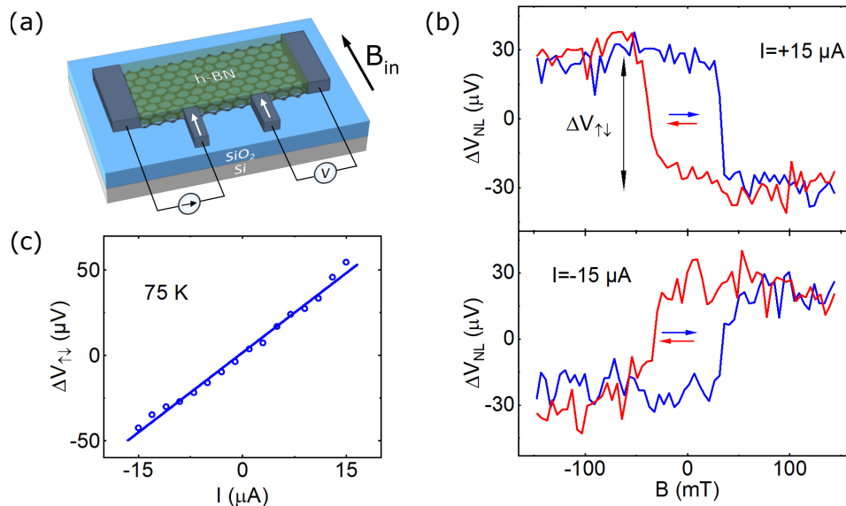
Figure 3.6: (a) Schematic of the nonlocal measurement configuration. (b) Measured nonlocal voltage V_{NL} as a function of external in-plane magnetic field ( B_{||} ) at I = \pm 15 \mu\text{A} at 75 K. The B_{||} sweep directions are indicated by red and blue arrows. A baseline linear background voltage is subtracted from the measured data. (c) Current bias dependence of the magnetoresistance switching amplitude \Delta V_{\uparrow\downarrow} at 75 K.
