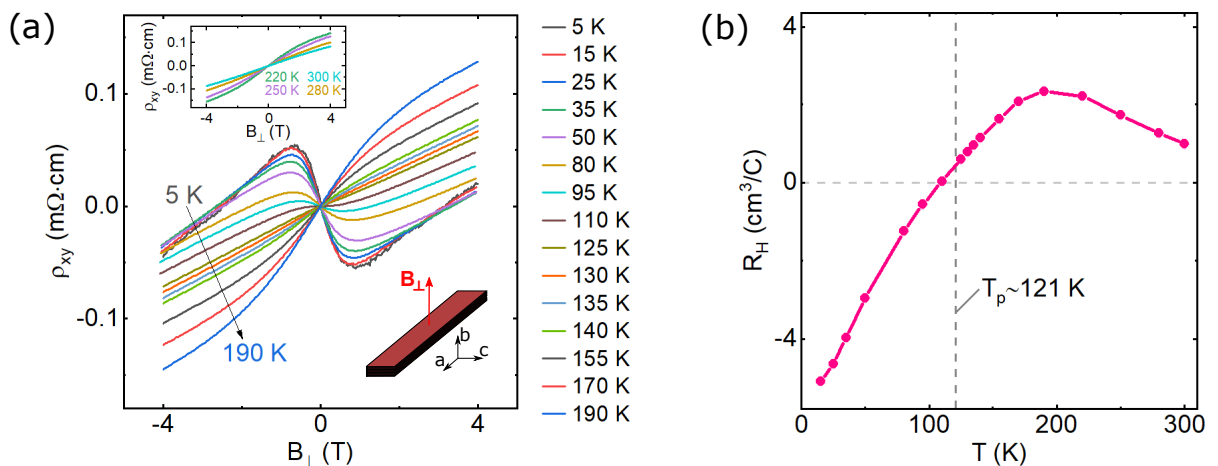
Figure 5.9: (a) Temperature dependence of the Hall resistivity \rho_{xy} in \text{ZrTe}_5 in the range of 5-190 K (main panel) and 220-300 K (top inset). Bottom inset indicates direction of applied magnetic field with respect to the flake crystal axes. (b) Hall coefficient R_H as a function of temperature. The vertical dashed line marks the position T_p of the resistivity anomaly peak.
