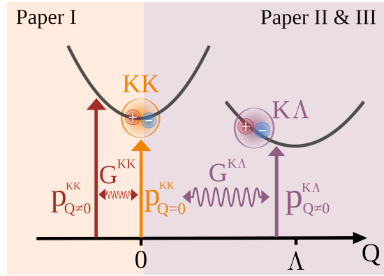
Figure 4.2: Intravalley and Intervalley coupling. Excitonic dispersion of K and \Lambda valley. The external electromagnetic field drives the excitonic resonances p_{\mathbf{Q}=0}^{\text{KK}} which can couple via the molecules either with polarizations p_{\mathbf{Q}\neq 0}^{\text{KK}} within the same valley (orange) or with polarization p_{\mathbf{Q}\neq 0}^{\text{K}\Lambda} in the \Lambda (purple) valley, intra and intervalley coupling respectively.
