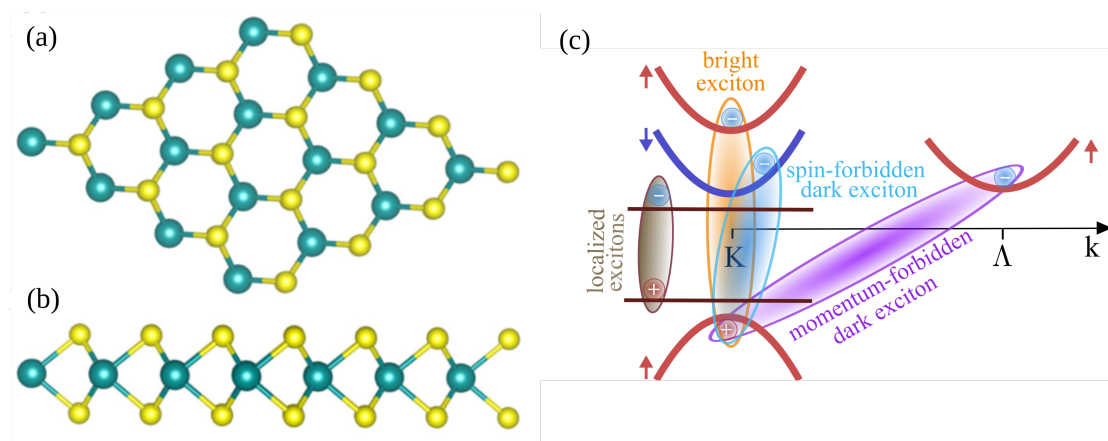
Figure 1.1: Schematic view of a TMD monolayer and the variety of excitons. (a) Top and (b) side view of a transition metal dichalcogenide monolayer, with blue representing M=(\text{Mo}, \text{W}) atoms and yellow representing X=(\text{S}, \text{Se}) atoms. Both M and X layers exhibit a honeycomb-like structure, similar to graphene. Figure taken from [2]. (c) Electronic dispersion around the high symmetry K/\Lambda points in the Brillouin zone. Beside bright excitons (yellow), where both electron and hole have the same spin and momentum, there also exist dark (not optically active) excitons. Dark states can be either spin (blue) or momentum (purple) forbidden. Besides, due to local changes in the band structure, states can appear within the band gap which give rise to the formation of localized excitons (brown). Figure taken from [3].
