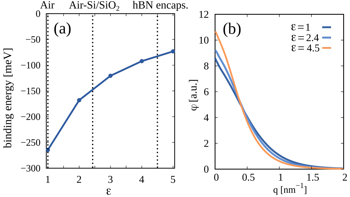
Figure 7.3: Excitonic eigenvalues and eigenfunctions of interlayer excitons for different dielectric screening. (a) The eigenvalues (= excitonic binding energies) of interlayer excitons show a decreasing behaviour with higher dielectric background \epsilon due to stronger screening. (b) The eigenfunctions (=excitonic wave functions) become narrower in momentum space with higher screening and hence less localized in real space. Figure adopted from PAPER VIII.
