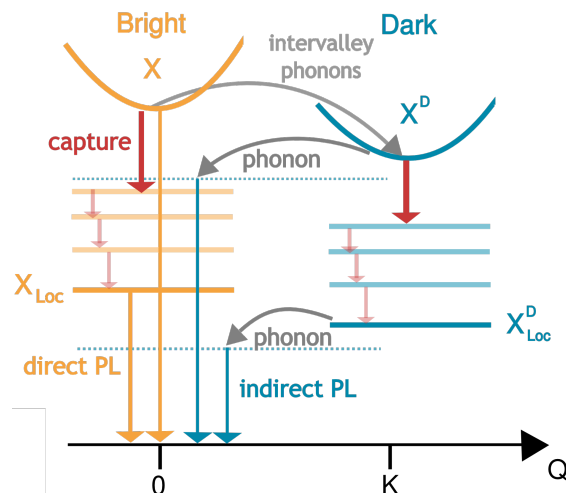
Figure 6.6: Relaxation and capture processes. Phonon-driven relaxation and capture processes involving both bright X and momentum-dark X^D excitons as well as their localized states X_{\text{Loc}} and X_{\text{Loc}}^D , respectively. We include phonon-assisted intervalley scattering, capture and relaxation of excitons as well as direct and phonon-assisted photoluminescence. Taken from PAPER VI
