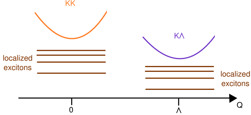
Figure 6.3: Excitonic dispersion with localized states. Illustration of excitonic dispersion, including free excitons with a parabolic dispersion as well as quantized localized excitons. Both KK and KΛ can be trapped, resulting in different energies of the corresponding localized states.
