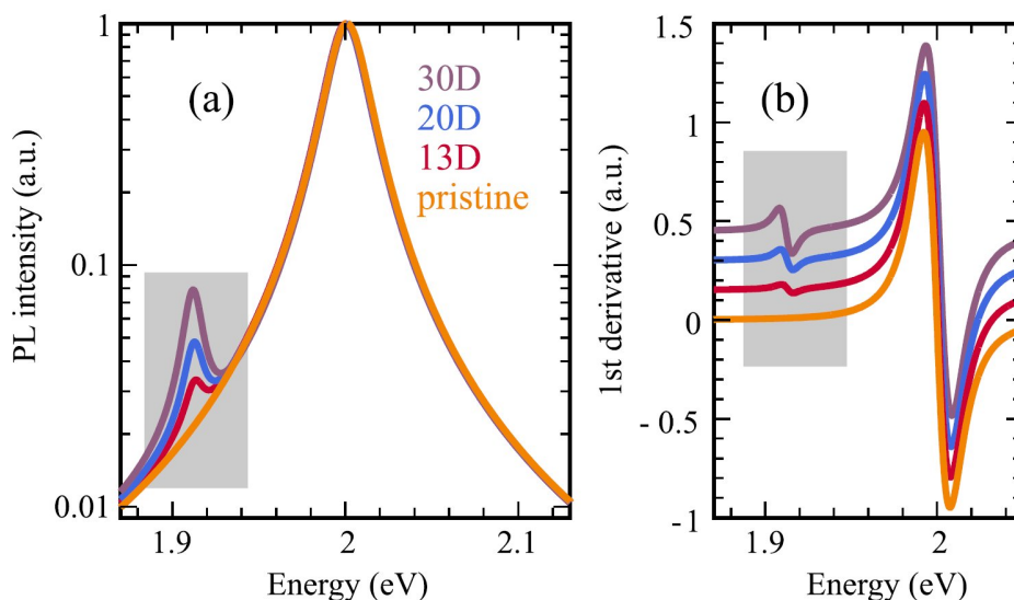
Figure 4.7: Room-temperature conditions. (a) Room-temperature PL in logarithmic plot and (b) first derivative of the PL in functionalized and pristine WS 2 for different dipole moments. The PL is normalized to the bright peak. We find that the visibility of the dark peak is in the range of 3-9 % compared to the bright peak. The main limiting factor is the broad excitonic linewidth at room temperature. Hence, we also show the derivative of the PL which shows clear traces of the dark exciton at room temperature even for 13 D. Note that the spectra are shifted along the y axes for better visibility. Figure taken from PAPER III.
