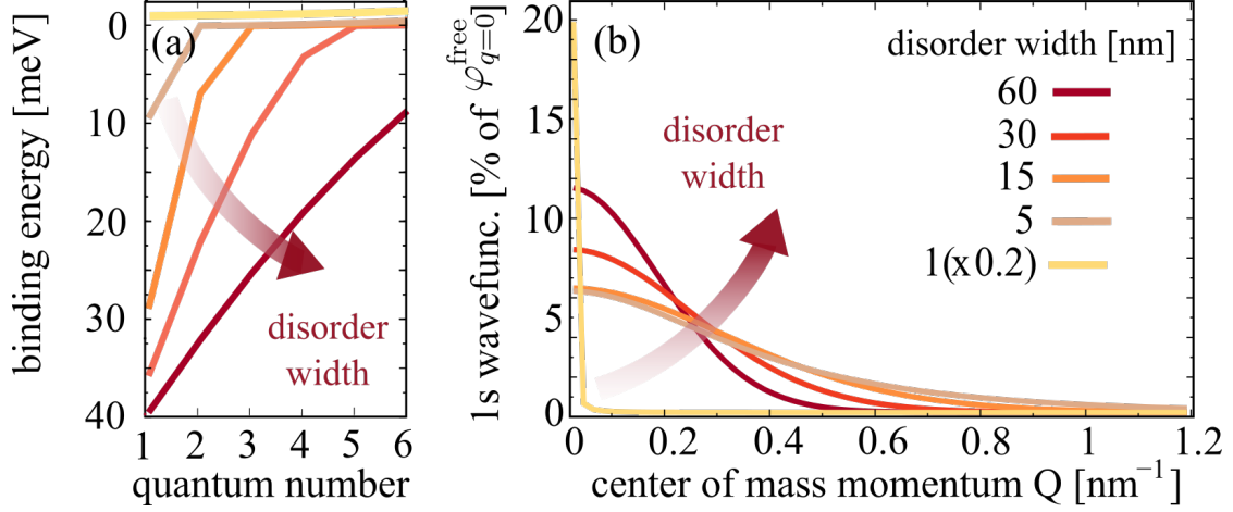
Figure 6.4: Characteristics of localized excitons. Disorder-width dependent (a) binding energies and (b) 1s wavefunctions of localized excitons. The broader the disorder potential, the more localized states exist and the stronger is their binding energies. Taken from PAPER VI
