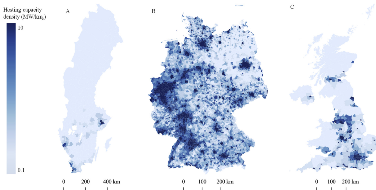
Fig. 5. Hosting capacity density map (MW/km 2 ) aggregated to local administrative units. Darker colours represent larger hosting capacity density. The colour scale is logarithmic to account for the large variation in hosting capacity density. Results shown for Sweden (A), Germany (B), and the United Kingdom (C). Note due to rounding error in the GIS aggregation, summation of hosting capacity density might not correspond to national hosting capacity.
