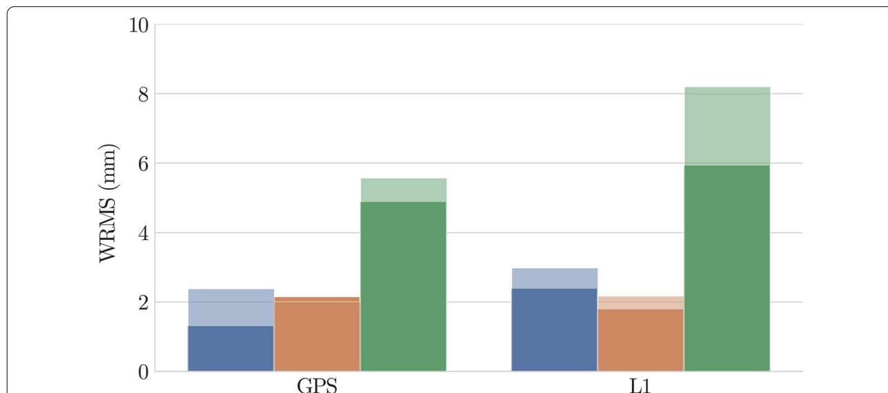
Fig. 5 Average station position repeatabilities (WRMS in mm) for the two co-located networks (VLBI L1 sites on the right and GPS sites on the left) for a single-technique solutions, i.e., sol-V and sol-G, (faded) and b the combined solution sol-VG (colored). The results are computed based on the 15 daily solutions. The components evaluated are north (blue), east (orange) and up (green) of the local topocentric frame
