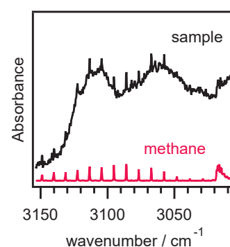
Figure 4.5: Methane peaks observed in the conversion stream for H-BEA SAR38 at 500 °C.
