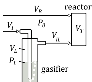
Figure 3.5: Volume flows using the gasifier setup.
