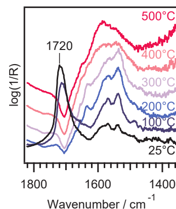
Figure 4.18: The region between 1800\text{ cm}^{-1} to 1400\text{ cm}^{-1} during a temperature-programmed DRIFTS experiment with 2,5-dmf and H-BEA. Difference spectra, background at 25^\circ\text{C} .
