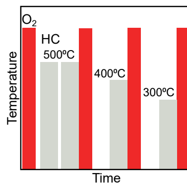
Figure 4.10: Experiment sequence: Catalyst calcination under 20% oxygen at 700 °C, HC pulses of 2,5-dmf at 500 °C, 400 °C and 300 °C.
