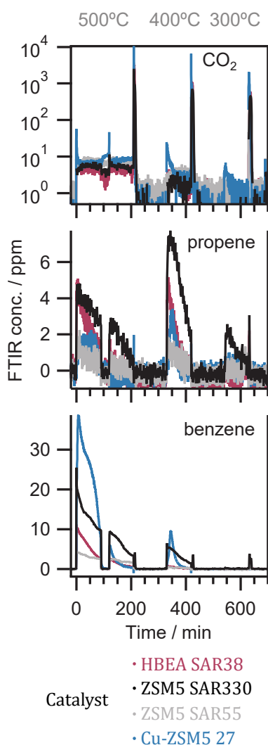
Figure 4.12: Concentration profiles of CO 2 , propene and benzene.
