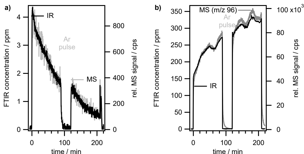
Figure 4.8: Comparison of FTIR and MS: Signal match of IR and MS for a) ethene ( m/z 27) and b) 2,5-dimethylfuran ( m/z 96).
