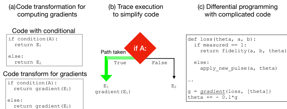
Figure 3.2: Differential programming requires automatic differentiation of computer programs. (a) Code transformations produce a code with similar conditionals as the input program for the gradients. (b) Execution-trace-based automatic differentiation uses a trace of the program that does not contain the conditionals since at execution, a computer code is a sequence of well-defined steps. (c) Differential programming could enable writing computer programs that can be treated in a similar way to neural networks and learned by training on data.
