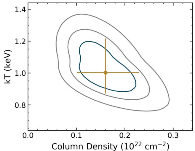
Figure 9. Best-fit confidence map for the plasma temperature ( kT ) and column density ( N_{\text{H}} ) of the X-ray spectral fit. The best-fit solution is depicted with a 98% confidence range, and 68%, 90%, and 98% confidence levels are depicted.
