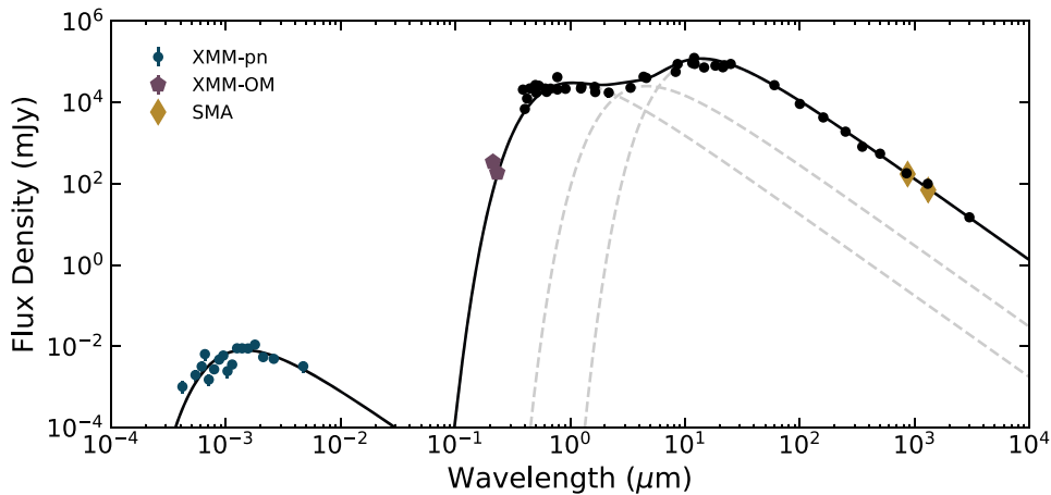
Figure 5. SED for U Mon. Representative archival data (black points) were collected from VizieR and the Herschel archives, as well as the 850\ \mu\text{m} measurement from de Ruyter et al. (2005) and the 1.3 and 3 mm measurements from Sahai et al. (2011). We present the new XMM-pn spectrum in teal points, the XMM-OM data in pentagons, and the SMA data in diamonds. The scatter in the archival data is probably due to intrinsic (pulsation or RVb) variability of U Mon at the time of observation. Note: error bars are smaller than the symbols.
