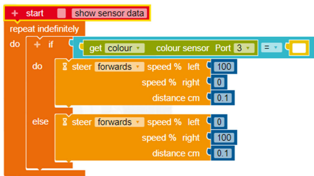
Fig. 1 Block-based mission of a robot patrolling a perimeter wall, expressed in Open Roberta
