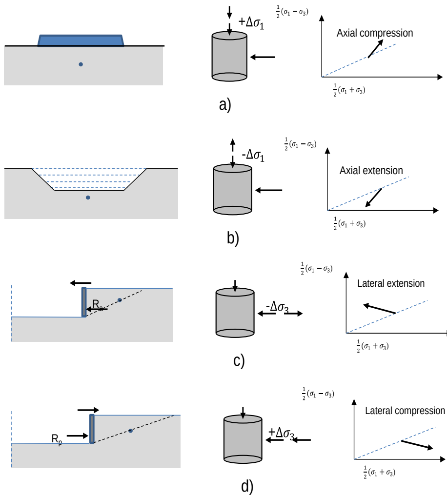
Figure 1. Example total stress paths a) Under centreline of an embankment or footing; b) At the bottom of a cut excavation; c) Behind a retaining wall when the wall is moving away from the soil (active earth pressure); and d) Behind a retaining wall when the wall is moving towards the soil (passive earth pressure).
