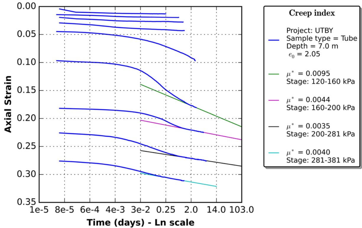
Figure 22. Modified creep index \mu^* for Utby clay.
