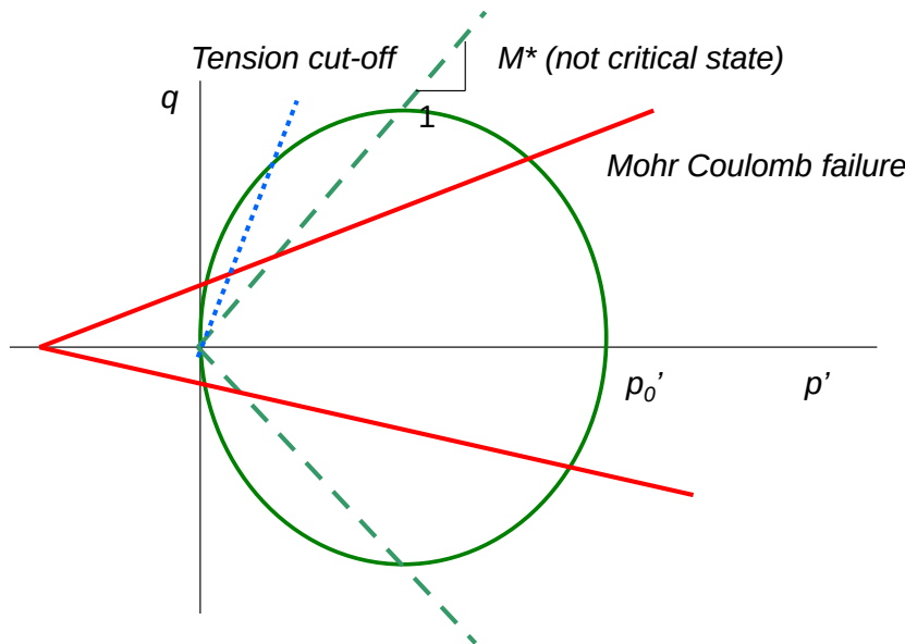
Figure 4. Soft Soil model.
