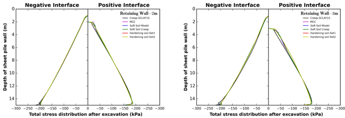
Figure 47. Predicted total stresses for 2 m deep excavation (left) and for 3 m deep excavation (right).
