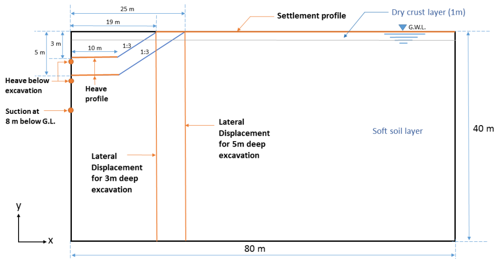
Figure 37. Benchmark cut excavation.
