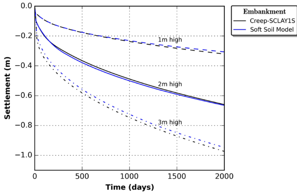
Figure 34. Predicted settlements under the centreline of the embankment on Utby clay for three different embankment heights.
