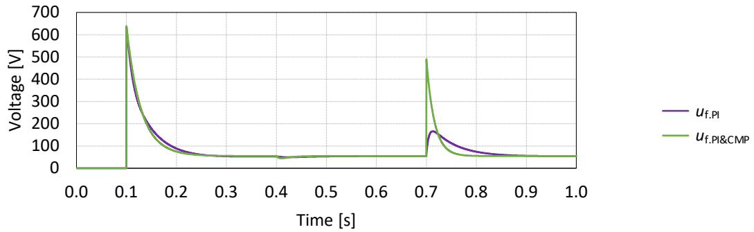
Figure 4-12 Waveforms of field voltage.
