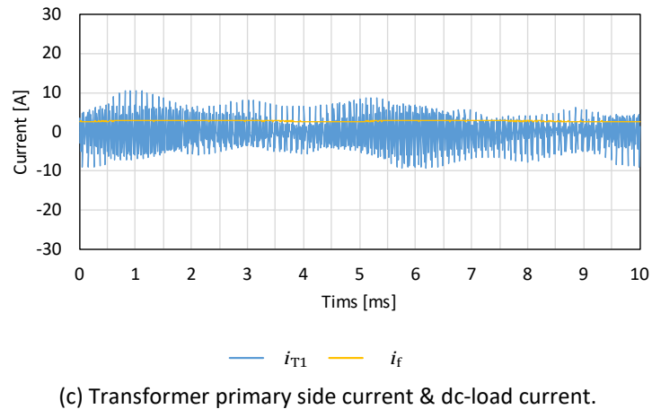
Figure 6-51 Time-domain waveforms m_a = 0.5 , k_7 = 0.0 , \alpha = 0^\circ .
