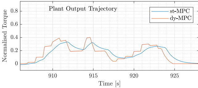
(b) Effect of dynamics ( @\tau_{ice} = 1 s) on the optimal ICE torque, optimal control input and ICE plant output trajectories. Dy-MPC delivers an optimal control policy whereas st-MPC struggles due to actuator dynamics mismatch.
