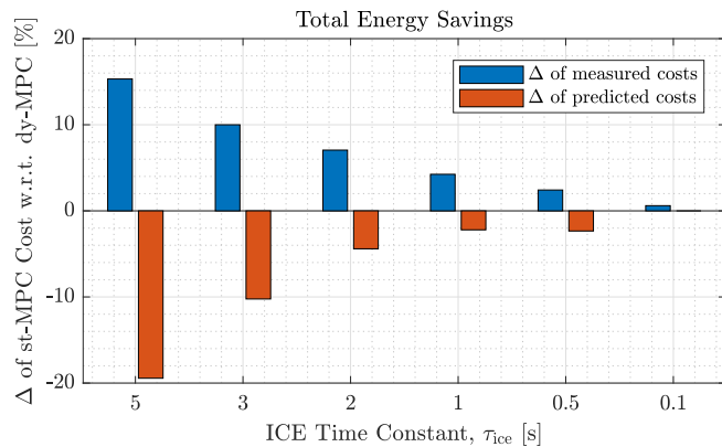
Fig. 5. Percentage variation in the total energy consumption (arithmetic sum of variations of the cumulative fuel and battery energy consumption) of the st-MPC w.r.t dy-MPC under different levels of ICE dynamic response tuning. The result shows that the dy-MPC can maximise energy savings when the actuator dynamics are increasing sluggish in nature, for the considered HEV powertrain configuration.
