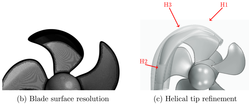
Figure 2: Mesh distribution of the propeller.
