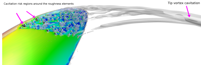
Figure 6: Distribution of the vortical structures around the roughness elements along with the iso-surface of pressure colored black, zoomed view of the roughness elements on the SS.
