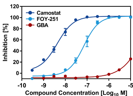
Fig. 4. Camostat mesylate and FOY-251 inhibit the activity of recombinant TMPRSS2. Incubation of recombinant TMPRSS2 with the Boc-Gln-Ala-Arg-MCA peptide substrate leads to the cleavage of the substrate and the release of the AMC(7-Amino-4-methylcoumarin) fluorophore, resulting in a fluorescent signal. Data were normalized against the fluorescence signals obtained in the absence of test compounds (Camostat mesylate, FOY-251, GBA). The concentration-response data for each test compound were plotted and modeled by a four-parameter logistic fit to determine the 50% effective concentration (EC 50 ) value. Inhibitory activity of Camostat mesylate (blue), FOY-251 (light blue) and GBA (red) against TMPRSS2 recombinant protein were visualized and curve fitting was performed using GraphPad Prism. The average of two biological replicates, each performed with four (Camostat mesylate and FOY-251) or two technical replicates (GBA) is shown. EC 50 values were 4 nM (Camostat mesylate), 70 nM (FOY-251), >10 \mu M (GBA).
