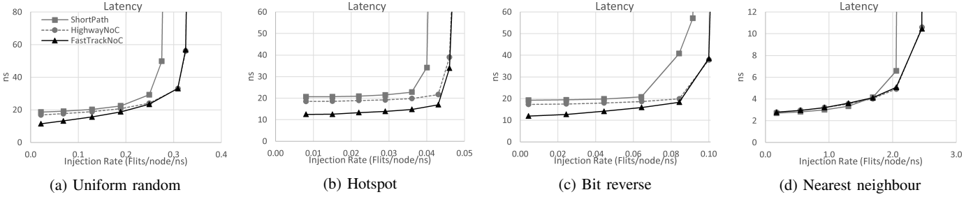
Fig. 10: Average packet latency of 32×32 2D mesh networks for 4 different traffic patterns.
