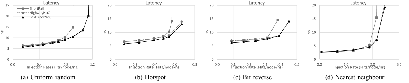
Fig. 8: Average packet latency of 8×8 2D mesh networks for 4 different traffic patterns.
