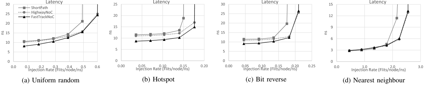
Fig. 9: Average packet latency of 16×16 2D mesh networks for 4 different traffic patterns.
