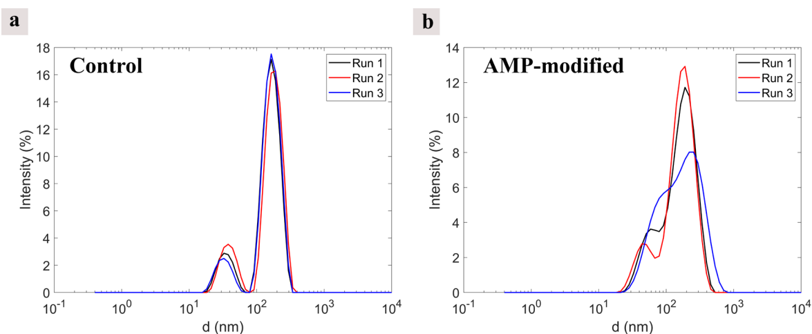
Figure 10. Size distributions (intensity-based) measured by DLS of the filtrated ( <6 \mu\text{m} ) particles. (a) The size distribution of non-modified control particles over three consecutive 60 second runs. (b) The size distribution of the AMP-modified particles over three consecutive 60 second runs.
