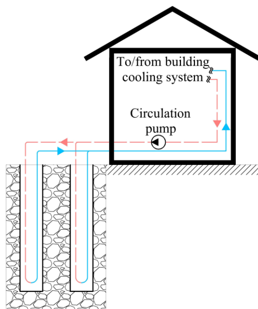
Figure 1.1. Schematic of a DGCS using vertical GHEs.
