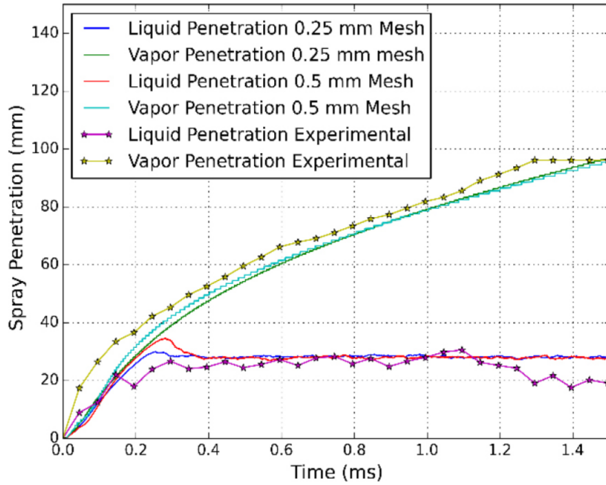
Figure 5.2: Comparison of spray penetration for a fine and coarse mesh.
