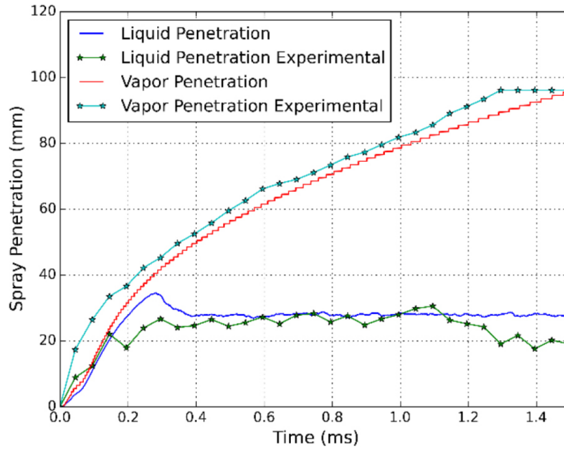
Figure 5.4: Spray penetration of the ethanol spray using the VSB2 spray model with tuned coefficients in the turbulence model.
