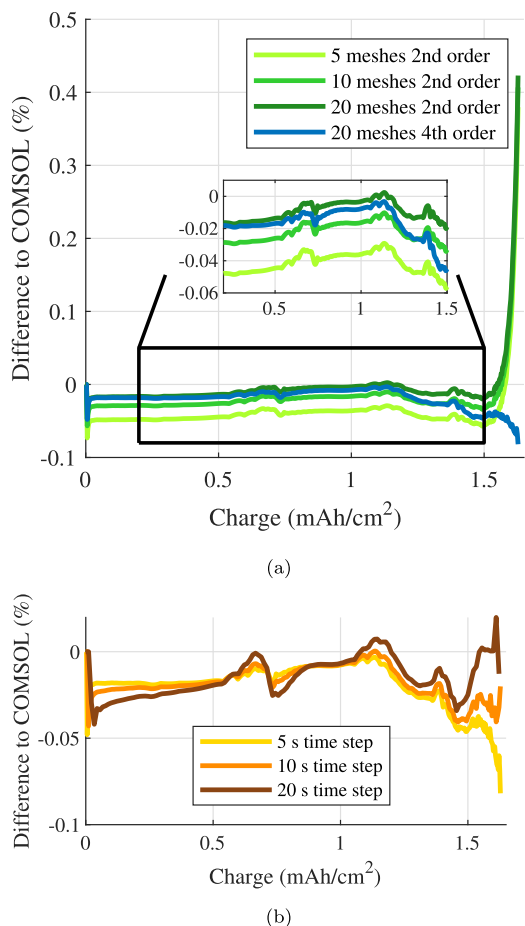
Fig. 7. Performance of the model with different meshing sizes and different time steps under a discharge current density of 2 mA/cm 2 .
