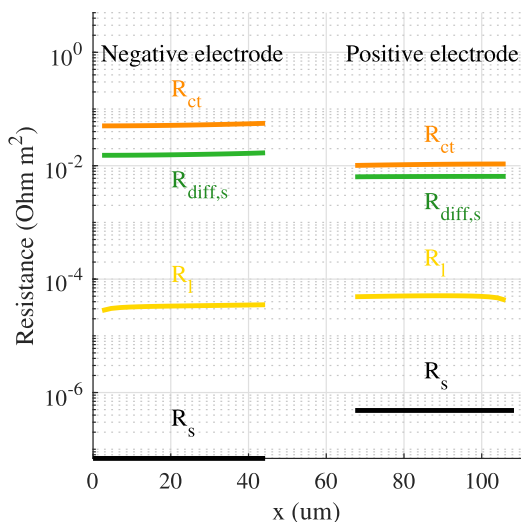
Fig. 9. The resistance values in the transmission line structure when the cell voltage is discharged to 3.6 V under a discharge current density of 2 mA/cm 2 . 20 mesh elements are used in each electrode. The y-axis is in logarithmic scale.
