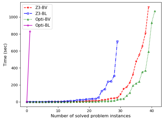
Fig. 1: Performance comparison between bit-vector (BV) and boolean (BL) time-index models over the generated instances using Z3 and OptiMathSAT. The maximum time allowed for each instance is 1200 seconds.
