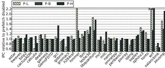
Figure 3: Performance impact of enabling prefetching relative to allocation of cache and bandwidth, for allocation settings; L:128kB,1GB/s B:512kB,4GB/s H:2MB,16GB/s
