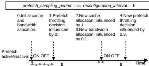
Figure 8: Timing and interactions of CBP resource manager.
