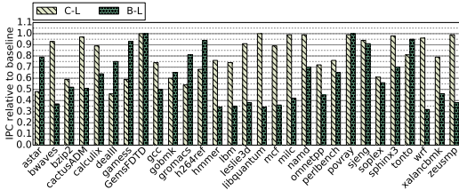
(a) Slowdown when decreasing the cache size to 128kB (C-L), and slowdown when decreasing the bandwidth allocation to 1GB/s (B-L) in comparison to the baseline allocation, with prefetching disabled.
