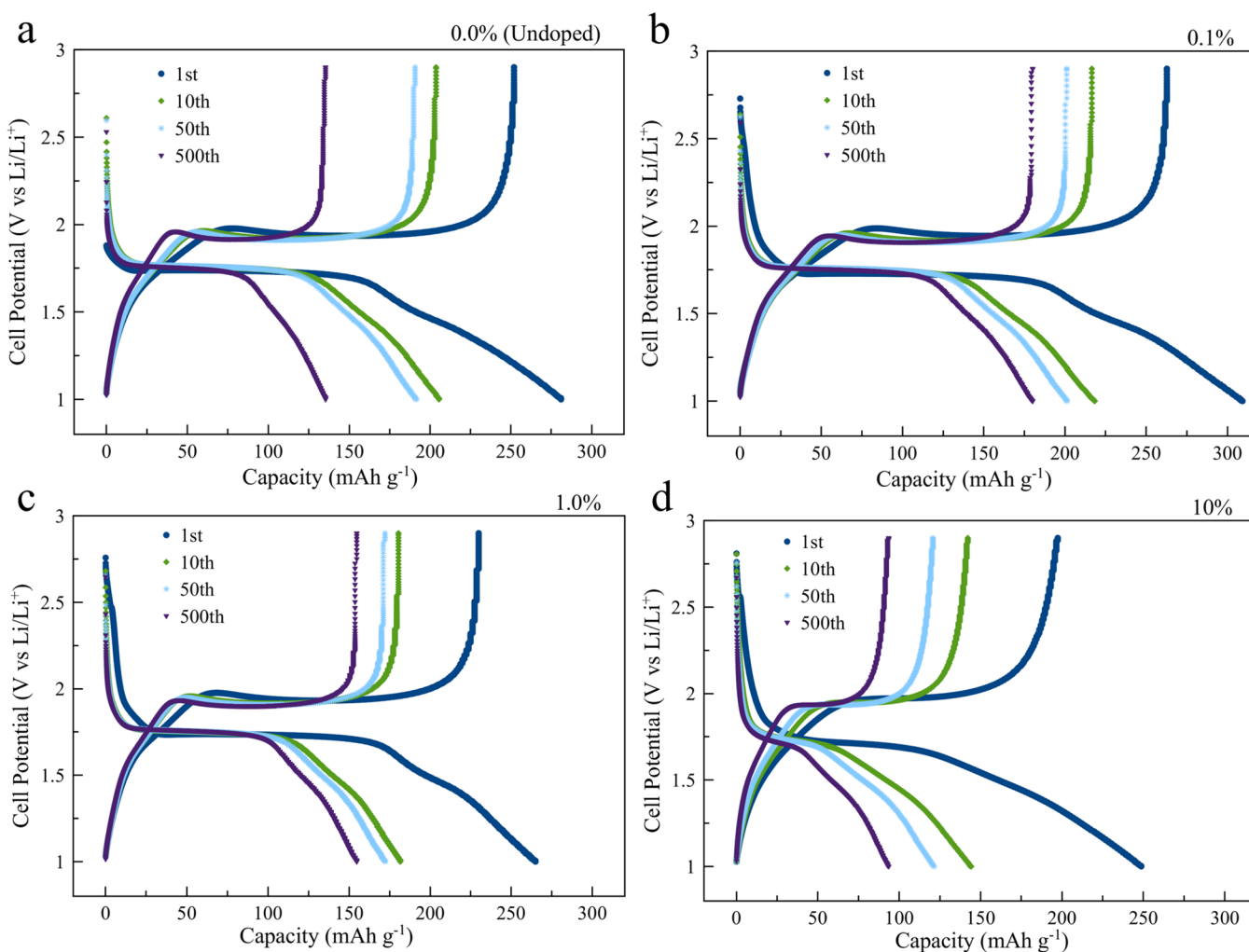
Figure 8. Galvanostatic charge/discharge curves at 1C: (a) undoped TiO 2 , (b) 0.1% at. Nb, (c) 1.0% at. Nb, and (d) 10% at. doping.
