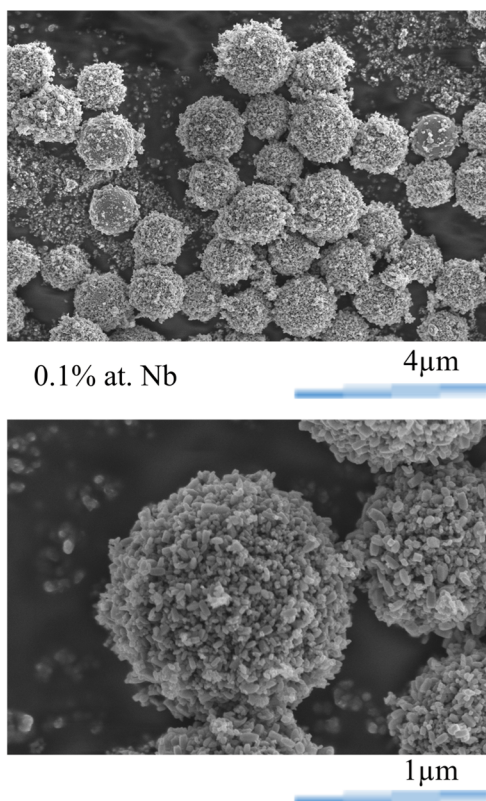
Figure 2. Scanning electron microscopy images of Nb-doped \text{TiO}_2 at 0.1% at. The higher magnification reveals the well-defined 3D hierarchical structure of the beads.
