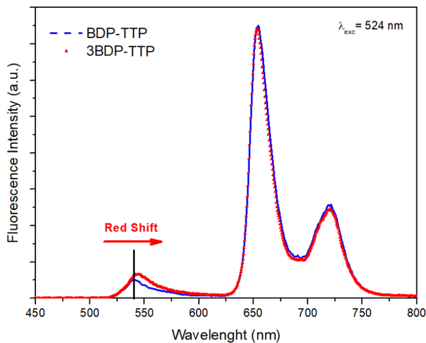
Figure 2. Emission spectra of BDP-TTP and 3BDP-TTP solutions in THF with the 524 nm excitation wavelength ( 2 \times 10^{-6} \text{ M} ).
