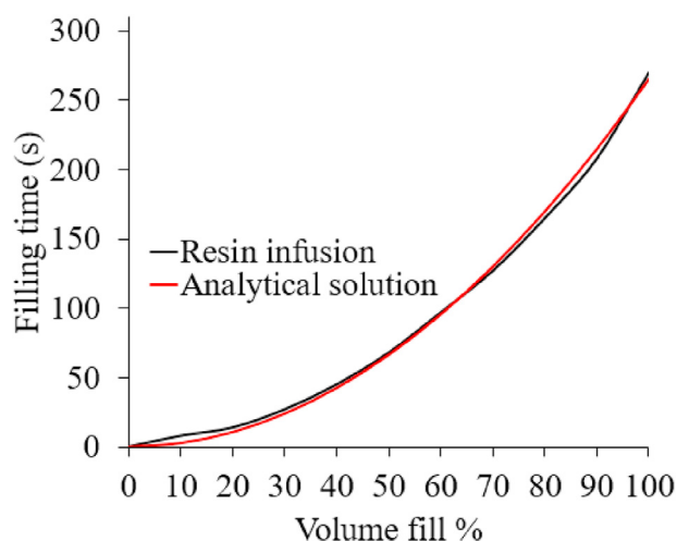
Fig. 9 – Comparison between experimental filling time and the analytical solution, Eq. (3).
