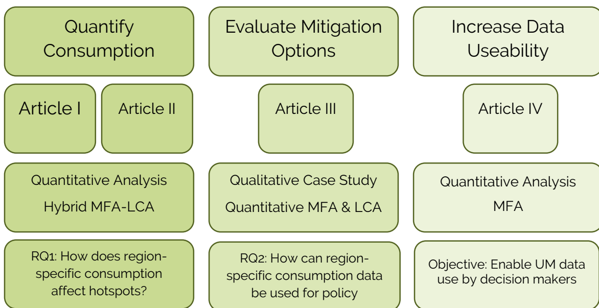
Figure 2. Research design
