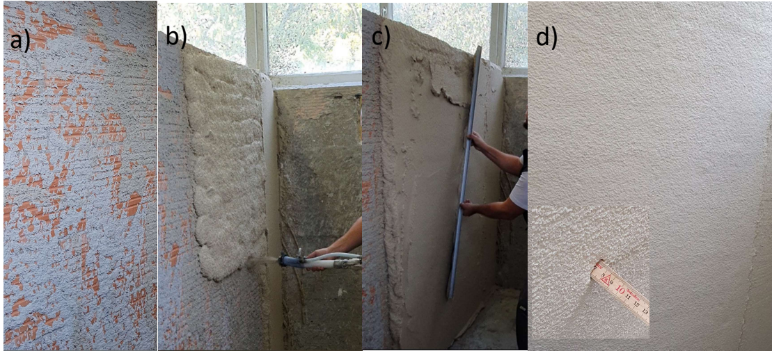
Figure 2. Photos showing the application steps of AP on a demo wall. a) Undercoat layer is smeared onto the surface. b) AP is sprayed on the surface until the desired thickness is achieved. c) The surface of the applied AP is smoothed. d) The final exterior appearance of the AP after the application.
