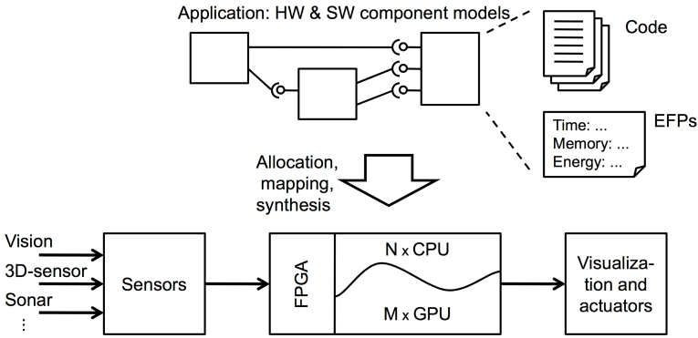
Figure 1.2: Generic modelling scenario of cyber-physical systems, depicting software deployment on a heterogeneous platform [10].
