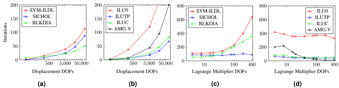
Fig. 1: Iterations required the GMRES method to achieve convergence for (a) fully monolithic - NBC, (b) linear multi-point constraints condensed method - NBC, (c) fully monolithic - varying \mathbf{t} discretisation, and (d) multi-point constraints condensed method - varying \mathbf{t} discretisation.
