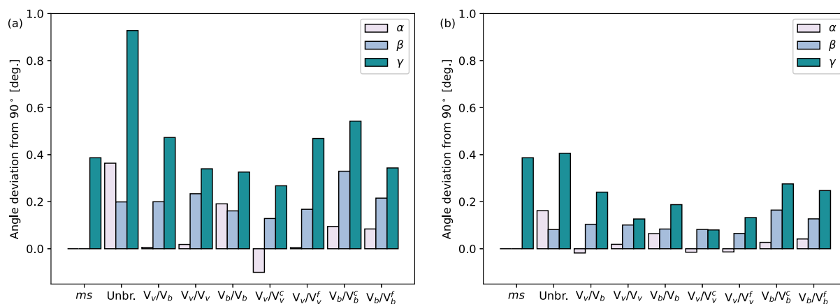
Figure 3. Cell vector angle deviations from 90° of (a) 2 \times 2 \times 1 (1.6% vacancy ratio, BiVO 3.9375 ) and (b) 3 \times 3 \times 1 (0.7%, BiVO 3.972 ) configurations.
