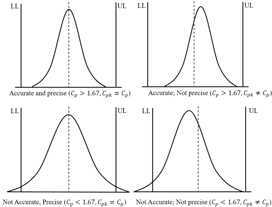
Figure 2.2: Difference between variation (accuracy) and the mean deviation (precision).
