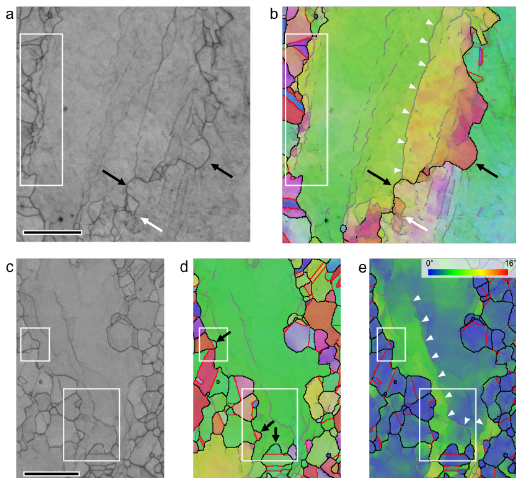
Figure 15. Nucleation of DRX grains. (a) Band contrast and (b) IPF maps from a sample deformed at 1080 °C and 0.05 \text{ s}^{-1} , showing bulging grain boundaries (black arrows) and misoriented subgrains along grain boundaries (white arrow and white rectangle). A long low angle boundary with misorientation in the range 5\text{--}7^\circ is indicated by multiple white arrowheads in (b). (c) Band contrast, (d) IPF and (e) grain reference orientation deviation (GROD) maps from same sample as in (a), showing “cutting off” of DRX grains by twinning (red lines in the white rectangles, also marked with black arrows in (d)), and concentration of deformation along grain boundary (multiple white arrowheads in (e)). Scale bar is 20 \mu\text{m} .
