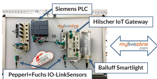
Real Industrial training system
