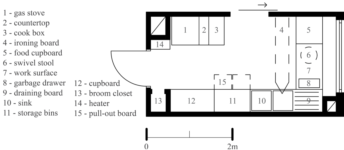
Figure 3 – Frankfurt kitchen designed by Margarete Schütte-Lihotzky, 1926 (adapted from Almqvist, 1940, pp. 28)
