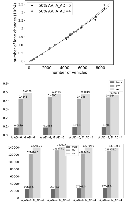
Fig. 14: Number of lane changes in simulations with different parameters' values. Top: number of lane changes as the number of vehicles varies. Middle and bottom: relative density (middle) and number of lane changes (bottom) for each type of vehicle (truck, AV and MV) for different values of the apparentDecel of MV ( M\_AD ) and AV ( A\_AD ).
