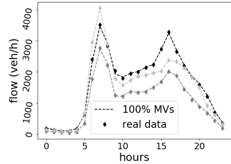
Fig. 2: Flow of vehicles as hours change (on August 29, 2002). The detections of the real devices (markers) are compared with the detections of the loops in SUMO (lines): device 1 (black), 2 (gray) and 3 (light gray).
