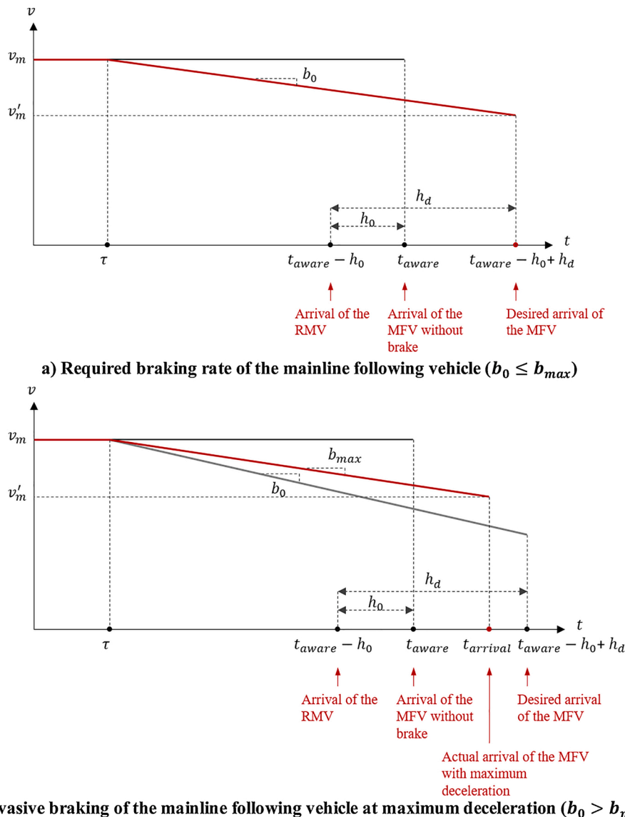
Fig. 6. Evasive braking rate of the mainline following vehicle.
