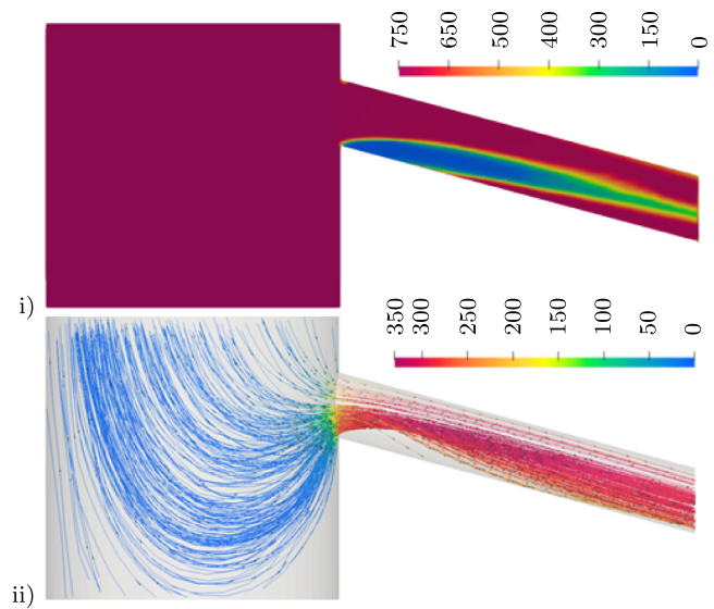
Fig. 12. Density distribution [kg/m 3 ] shown in a vertical section cut in the middle of the nozzle bore (side view) for the nozzle type N105 (i), while streamlines colored by velocity magnitude [m/s] give the flow path inside the nozzle (ii) taken at the end of the simulation.
