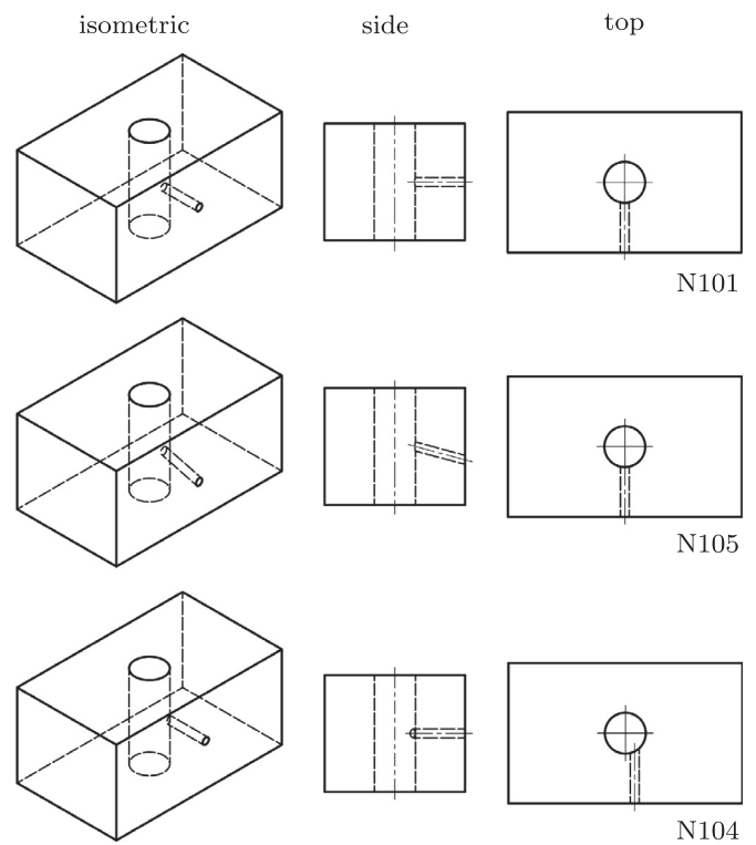
Fig. 3. Isometric, side, and top projection of the three different transparent nozzle types used. N101: centrally arranged 90° setup, N105: centrally arranged 75° setup, and N104: eccentrically arranged 90° setup. The main bore diameter is 3.5 mm and the nozzle bore diameter is 0.75 mm.
