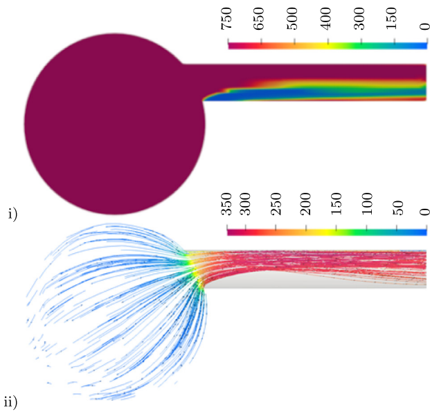
Fig. 11. Density distribution [kg/m 3 ] shown in a vertical section cut in the middle of the nozzle bore (top view) for the nozzle type N104 (i), while streamlines colored by velocity magnitude [m/s] give the flow path inside the nozzle (ii) taken at the end of the simulation.
