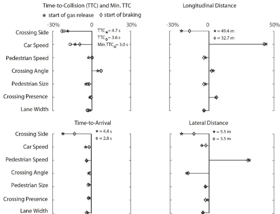
Fig. 5. Main factor effects from mixed effect models presented as percentage of the intercepts. Intercepts are also reported for start of gas pedal raelease and start of braking.
