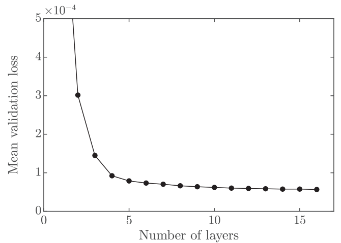
FIGURE 4 Minimum validation loss over 200 epochs, averaged over 20 runs for each number of layers, as a function of the number of layers
