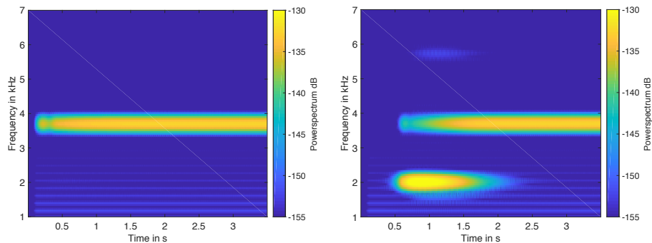
Figure 4. Spectrogram of the total displacement when the dither force starts immediately (left) and after 0.5 seconds (right). The dither frequency is 3606 Hz, the instability occurs at 2008 Hz
