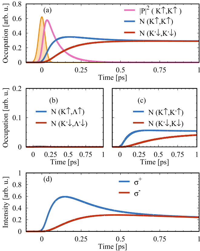
FIG. 2. Time evolution of exciton density and intensity of photoemission at 77 K in MoSe 2 . (a) illustrates the temporal evolution of K\uparrow, K\uparrow and K'\downarrow, K'\downarrow excitons. Additionally, we show the light pulse (yellow) as well as the optically injected excitonic transition (pink). (b) shows the temporal evolution of the K\uparrow, \Lambda\uparrow and K'\downarrow, \Lambda'\downarrow excitons. (c) shows the temporal evolution of the K\uparrow, K'\uparrow and K'\downarrow, K\downarrow excitons. In (d), we show the corresponding emission intensities of \sigma^+ and \sigma^- light.
