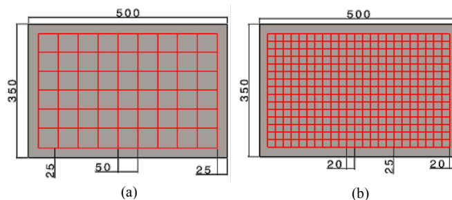
Fig. 4. (a) Heat treatment pattern A (b) Heat treatment pattern B
