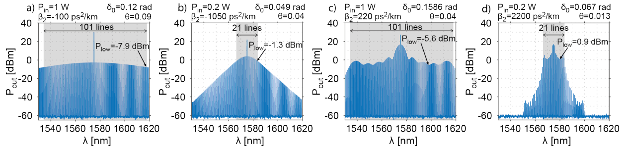
Fig. 2: a-b) show the optimal bright pulse combs for pump powers 1W and 0.2W, providing 101 lines and 21 respectively. c-d) show the optimal dark combs for the same number of lines and pump power as in a-b). One can deduce from the figures that using five 21 line combs (producing 105 lines) will result in a higher power per line than using a single 101 line comb, while the total optical pump power is the same in both cases.
