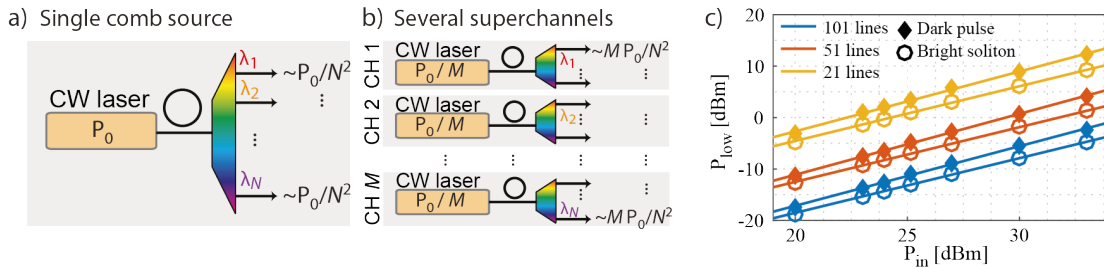
Fig. 1: The diagram in a) shows the single comb approach, providing N lines using a single comb and CW laser with pump power P_0 . In b) the total optical power has been distributed between M lasers, each pumping a separate comb providing N/M lines. According to the nonlinear scaling law this solution yields M times more power per line than the single comb. The graph in c) shows the simulated performance of individual combs generating N lines at different pump power, where P_{\text{low}} is the lowest power among these N lines. Each comb in the plot is found optimally in terms of group velocity dispersion, coupling rate and detuning. If we pick two combs that fit the approach in a) and b), e.g. 1 comb with 101 lines generated at P_{\text{in}}=30 dBm compared to M=5 combs with 21 lines generated at P_{\text{in}}=23 dBm, we see an improvement in performance by a factor M .
