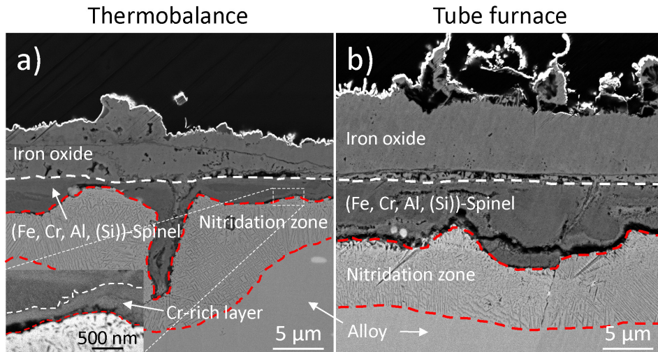
Figure 56: SEM cross section images of Fe15CrAlSi after exposure to 5% O 2 + 20% H 2 O + N 2 (bal.) in the presence of KCl at 600 °C in a) a thermobalance for 48 hours and b) a tube furnace for 168 hours.
