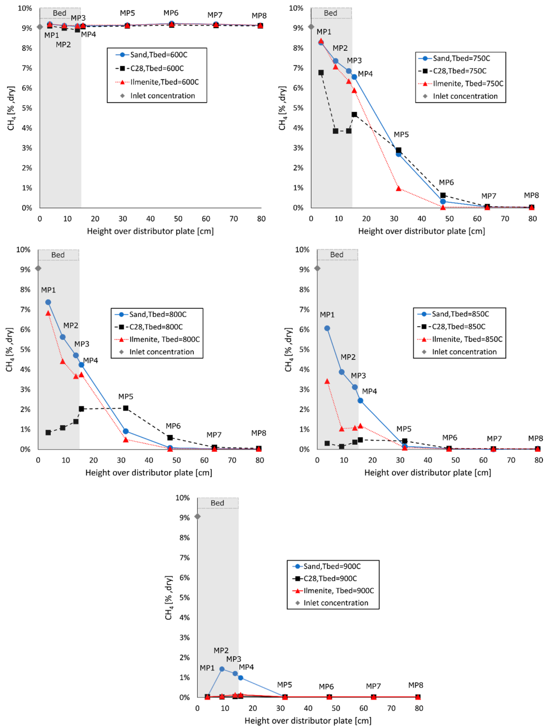
Figure 6. Measured gas concentration of CH 4 (in %, dry) at different distances from the distributor plate for all three bed materials where each subfigure presents a measurement at a certain bed temperature.
