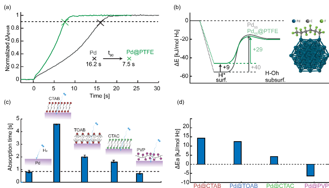
Figure 3: Polymer and surfactant/stabilizer effects on the hydrogen absorption rate in Pd. (a) Temporal response of neat Pd nanodisks and of Pd nanodisks coated with 50 nm PTFE to a 40 mbar \text{H}_2 pressure step. (b) Hydrogen absorption energy barrier of neat Pd and PTFE-coated Pd calculated with density functional theory (DFT). The used PTFE-Pd nanoparticle model is depicted in the inset ( Paper IV ). (c) Hydrogen absorption time for Pd nanodisks coated with the capping agents/surfactants CTAB, TOAB, CTAC, and PVP, respectively. Note that, as illustrated, the cationic head of the surfactant is attracted to the Pd surface while the ligand is facing away. The surfactants also form a bilayer structure on the surface. (d) Apparent hydrogen absorption activation energy change induced by the respective capping agent. ( Paper V ).
