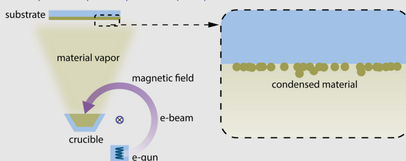
Scheme SI 3: Schematic of electron-beam physical vapor deposition (e-beam PVD). Electrons are generated by a heated-filament and directed by a perpendicular magnetic field onto the material source/crucible. The thereby heated material evaporates towards the substrate placed above the crucible in high vacuum. Material vapor adsorbs on the substrate and condenses and nucleates to form a thin film.
