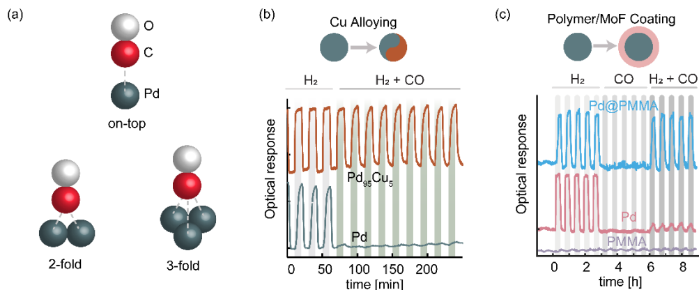
Figure 4: (a) Three different carbon monoxide adsorption geometries on Pd. Two strategies to mitigate CO poisoning on Pd: alloying with Cu (b) and polymer coating (c). (b) Temporal response of Pd and Pd 95 Cu 5 sensor to 4% H 2 and 4%H 2 +0.5% CO (in synthetic air background) at room temperature ( Paper II ). (c) Similar, temporal response of Pd and PMMA-encapsulated Pd to 10% H 2 , 0.5% CO, and mixture of 10% H 2 + 0.5% CO ( Paper VI ).
