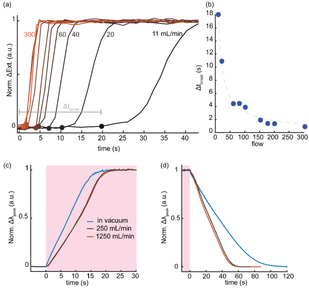
Figure 31: (a) Temporal optical \Delta\text{Ext} response of a 50 \mu\text{m} \times 0.0035 \text{ wt.}\% Pd:Teflon nanocomposite H 2 sensor to 100%-H 2 exposure in the fast-switch mini flow reactor at different flow rates: 11, 20, 40, 60, 80, 100, 150, 175, 200, and 300 mL/min. The synthetic air and 100%-H 2 valves were switched at t = 0 . Onset time ( \Delta t_{\text{onset}} ) is calculated from the time difference between the signal onset (signified by the dots) and t=0 . (b) \Delta t_{\text{onset}} vs. flow rate obtained from (a). The test was done at 25°C. (c) Absorption and (d) desorption temporal \Delta\lambda_{\text{peak}} response of a 190 nm \times 25 nm Pd@PTFE/PMMA sensor to 80 mbar H 2 (vacuum system) and 8 vol.% H 2 in synthetic air (fast-switch mini reactor). For the synthetic air background, two flow rates were tested: 250 and 1250 mL/min. The red shaded area denotes the H 2 exposure.
