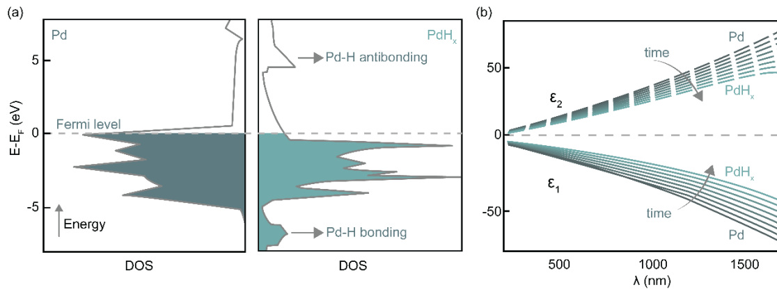
Figure 6: Pd and Pd-hydride electronic (a) and optical (b) properties. (a) The density of states (DOS) of pure Pd is characterized by the partially filled d-band, as denoted by the Fermi level. In the Pd-hydride, hydrogen atoms add more electrons to the system, thereby filling up the d-band. The Pd-H bonding and antibonding states are visible in the valence and conduction bands, respectively (adapted from ref. 151 ). (b) Dielectric function evolution during Pd-hydride formation. The real ( \epsilon_1 ) and imaginary ( \epsilon_2 ) part of the dielectric function are represented by the solid and dashed-lines, respectively (adapted from ref. 152 ).
