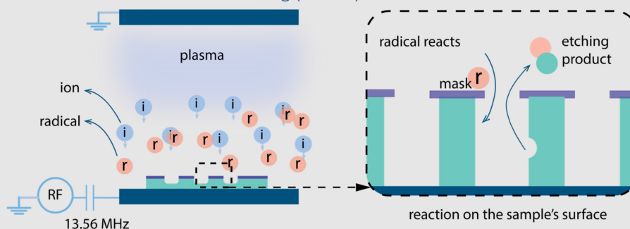
Scheme SI 2: Schematic of the plasma-enhanced reactive ion-etching process (adapted and modified from 256 ). Plasma is generated in between the two electrodes. The anode is connected to a radio-frequency generator. Plasma induces ion and radical formation in the feeding-gas (in my case O_2 for PMMA etching). In the inset, reactive radicals adsorb onto the sample surface to promote the etching reaction. In this case, I relate the illustration to the etching process of the PMMA sacrificial layer explained earlier in the hole-mask colloidal lithography section in Figure 17(g).
