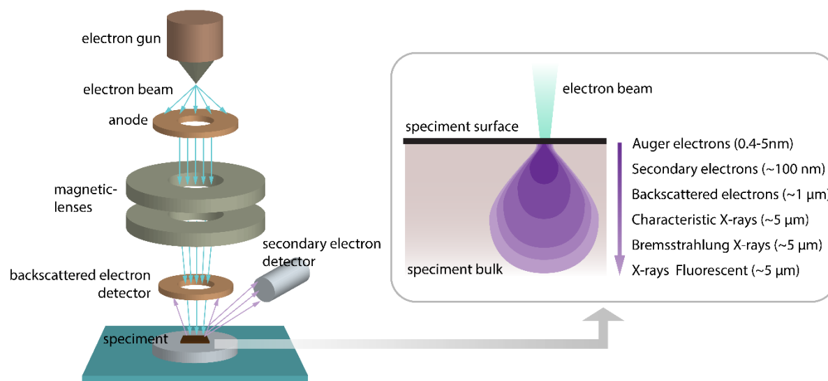
Figure 21: Schematic of a scanning electron microscope (SEM) (not to scale). The electrons are generated by an electron gun and then focused onto and rastered across the specimen by magnetic lenses. Inset: the profile of the generated signals from the specimen depending on the depth. For SEM imaging only the secondary and the backscattered electrons are used (adapted from refs. 236,237 )
