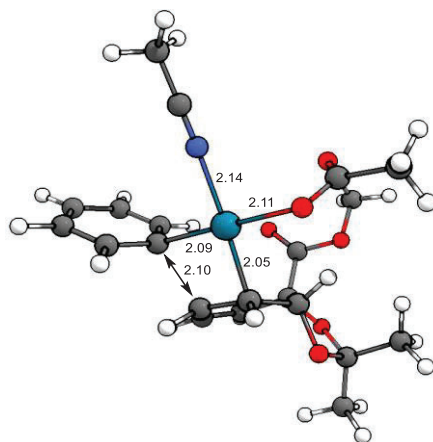
Figure 22 Optimized structure for migratory insertion transition state TS1 . Selected bond distances are shown in Ångström (Å).
