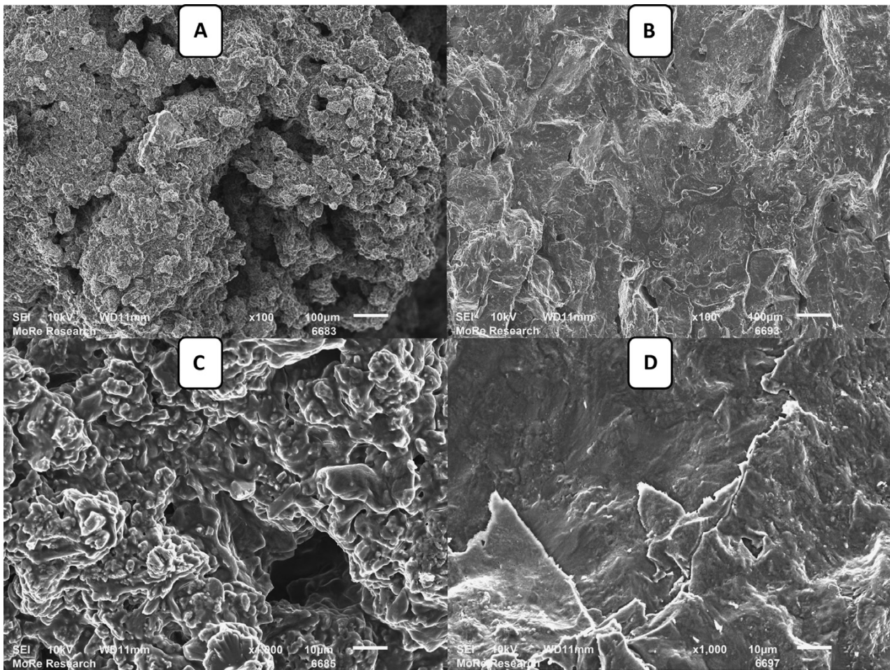
Figure 9: SEM secondary electrons images at 100 and 1000 \times magnification, of a fragment of black liquor scale from Sample 2 (A and C) and a fracture surface of salt solution scale from Sample 10 (B and D). The large voids in the black liquor scale fragment were probably formed when the fragment was broken.
