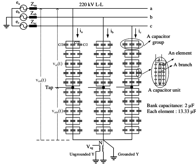
Fig. 4: A single Y-connected shunt capacitor bank.
