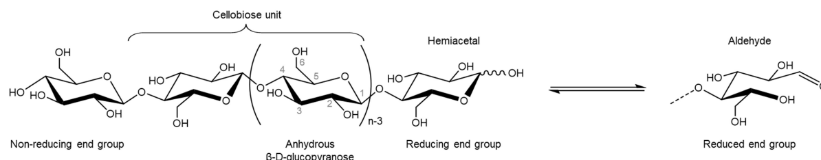
Figure 2.2. The molecular structure of cellulose, illustrating the repeating anhydrous glucose unit, the cellobiose unit and the non-reducing and reducing end groups as well as the equilibrium for reducing end group between the aldehyde and hemiacetal.
