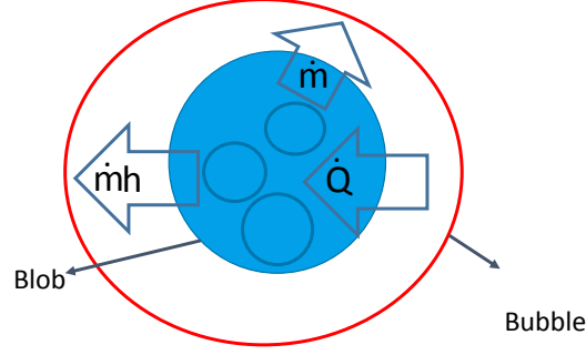
Figure 3.3: Evaporation of a blob in a bubble.
