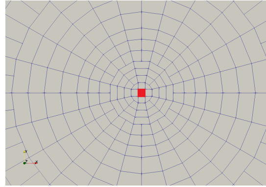
(b) Unresolved orifice, min grid size = 125 \mu m
