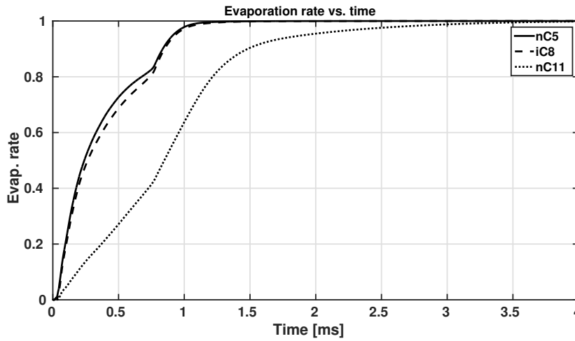
Figure 4.24: Individual evaporation rates for the three fuel components using the meshes with the counterbore.
