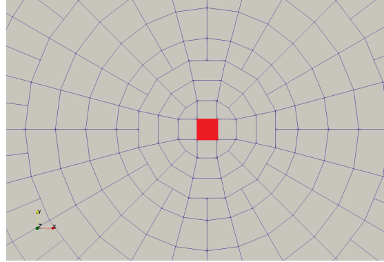
(c) Unresolved orifice, min grid size = 250 \mu m
