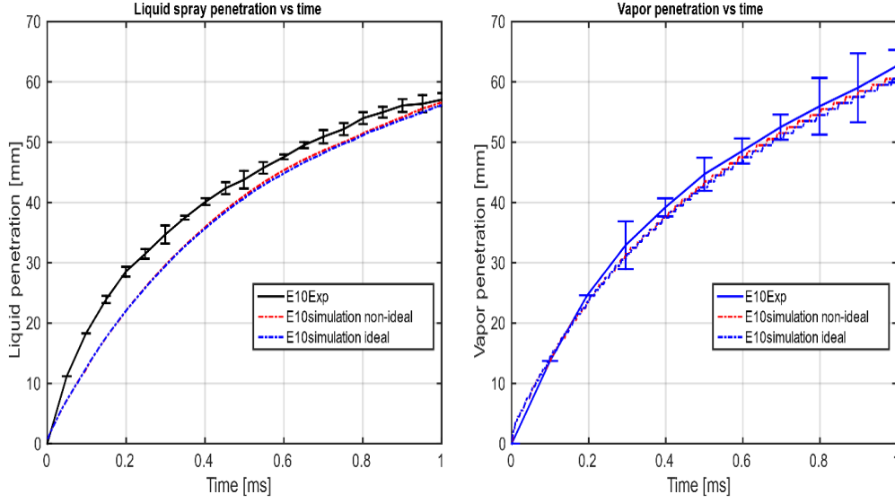
Figure 4.7: Liquid and vapor penetration vs. time for E10 case.
