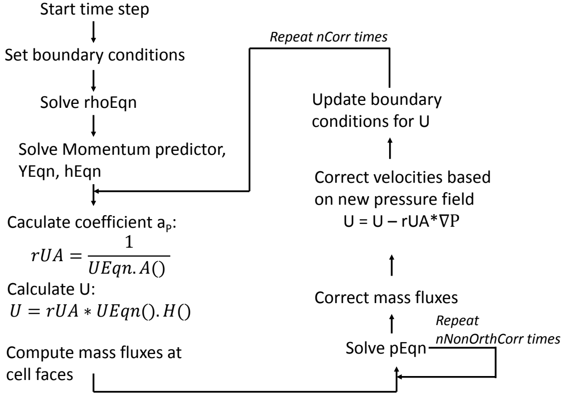
Figure 4.1: Solution algorithm.
