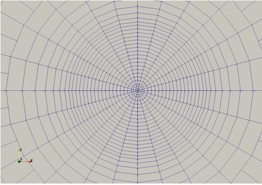
(a) Resolved orifice, min grid size = 28 \mu m
