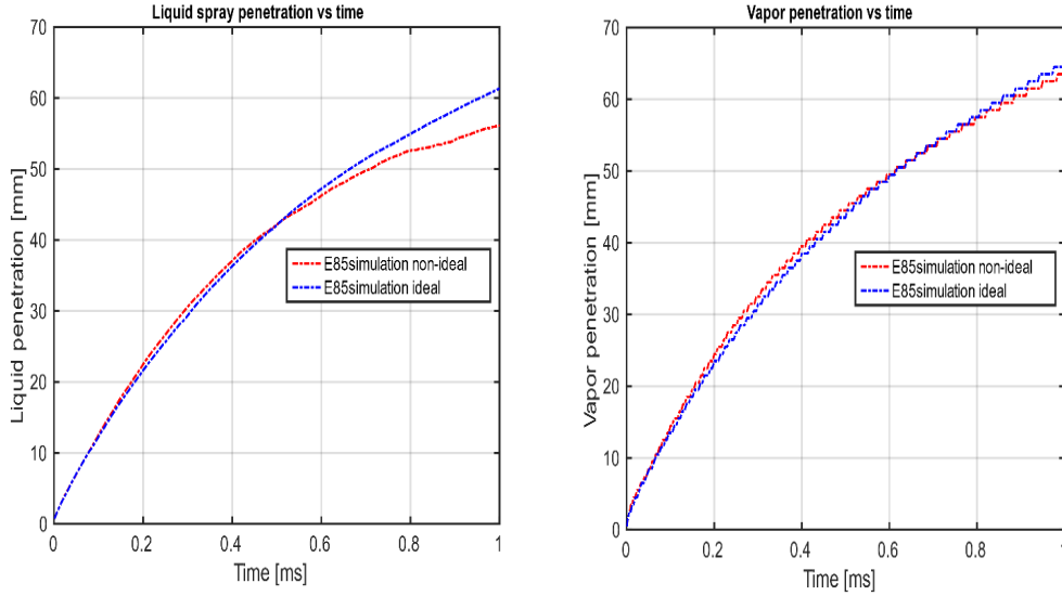
Figure 4.8: Liquid and vapor penetration vs. time for E85 case.
